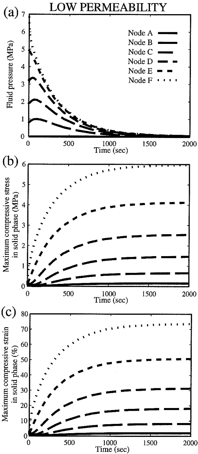
Figure 5. Time-dependent changes in (a) fluid pressure, (b) maximum compressive stress in the solid phase, and (c) maximum compressive strain in the solid phase for the low-permeability case. Locations of nodes A–F are shown in Figure 1.
